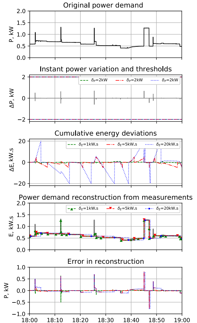
Fig. 1. Example of the EDM mechanism for arbitrary threshold values \delta_P = (2\text{kW}, 2\text{kW}, 2\text{kW}) and \delta_E = (1\text{kW.s}, 5\text{kW.s}, 20\text{kW.s}) . First top: original signal; second top: power variation; middle: cumulative energy deviations; second bottom: reconstructed signal from EDM; first bottom: error in the reconstruction. Adapted from [1].
