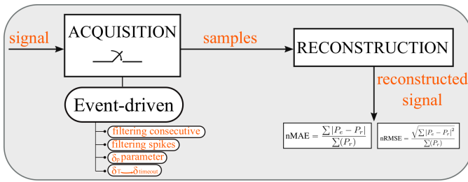
Fig. 2. Framework and functional blocks of EDM.
