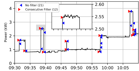
Fig. 5. Example of the consecutive-measurements filter. Source [1].
